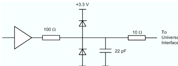
Circuit diagram of the output path
