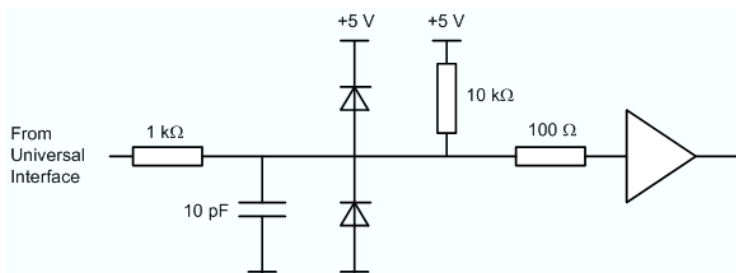
Circuit diagram of the input path
