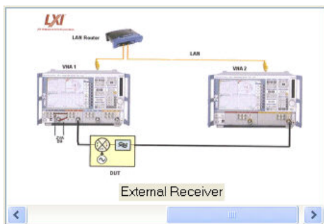
Test setup with external receiver
